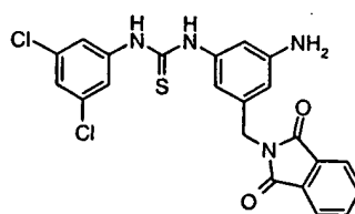
Compound # 31
